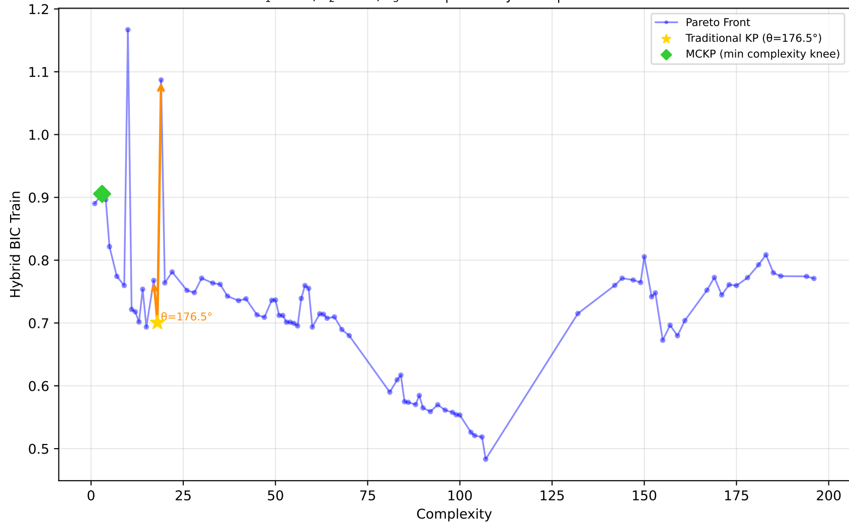
542_pollution - Run 10 - MVP - Hybrid BIC Train \lambda_1=0.40, \lambda_2=0.10, \lambda_3=0.00 | Difficulty: 1.00 | Method: hmr
