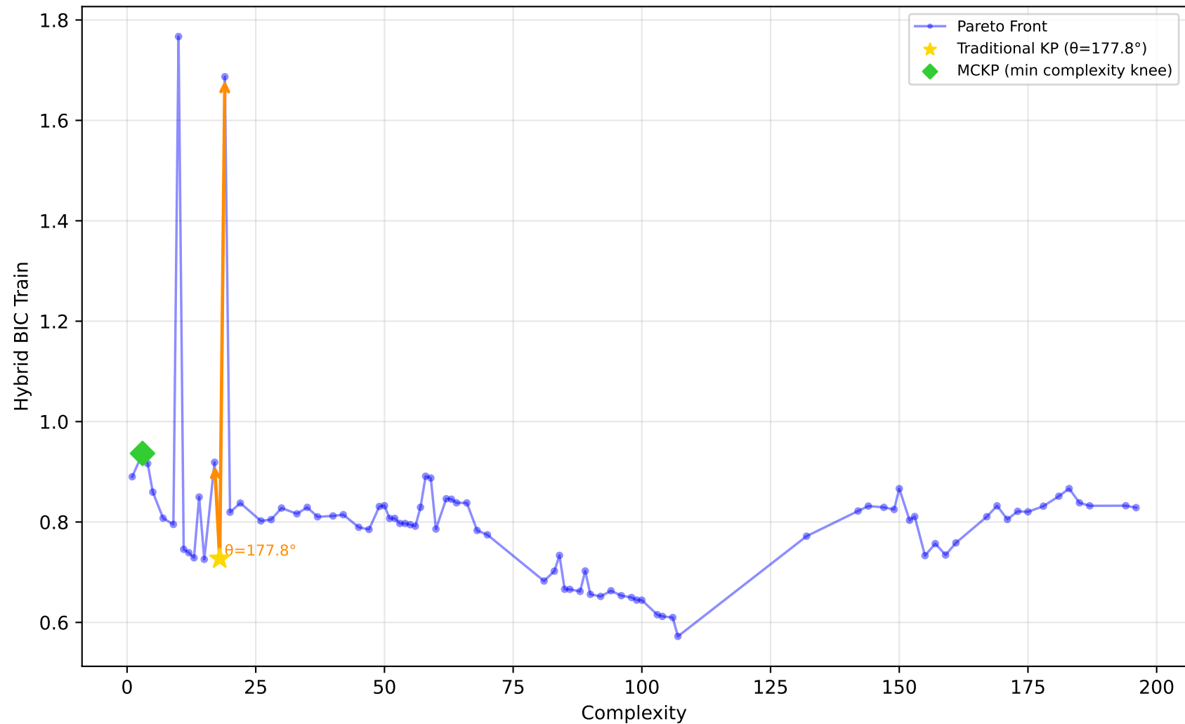
542_pollution - Run 10 - MVP - Hybrid BIC Train \lambda_1=1.00, \lambda_2=0.10, \lambda_3=0.00 | Difficulty: 1.00 | Method: hmr
