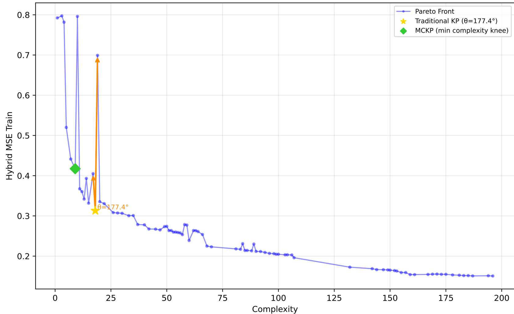
542_pollution - Run 10 - MVP - Hybrid MSE Train \lambda_1=0.40, \lambda_2=0.10, \lambda_3=0.00 | Difficulty: 1.00 | Method: hmr
