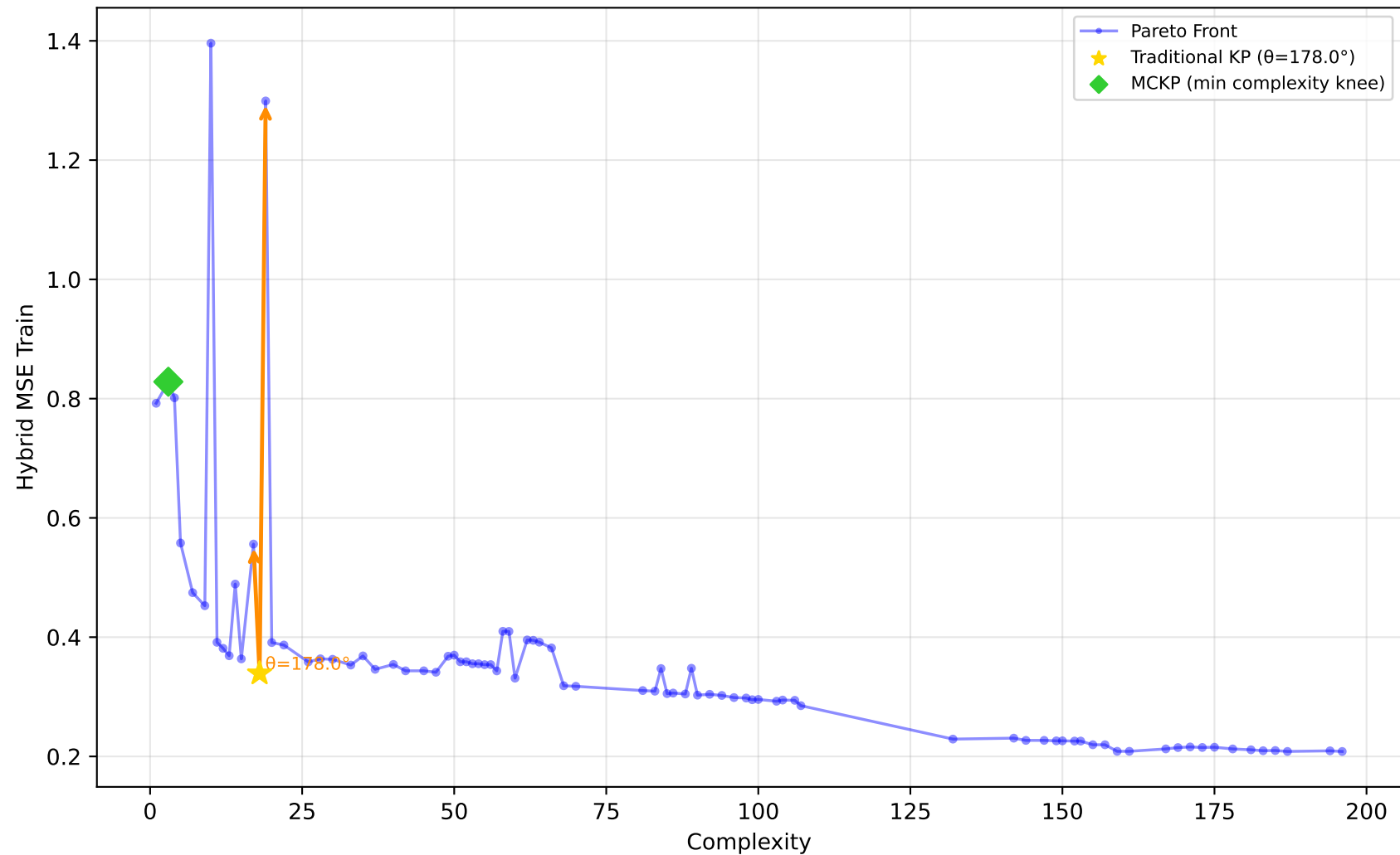
542_pollution - Run 10 - MVP - Hybrid MSE Train \lambda_1=1.00, \lambda_2=0.10, \lambda_3=0.00 | Difficulty: 1.00 | Method: hmr
