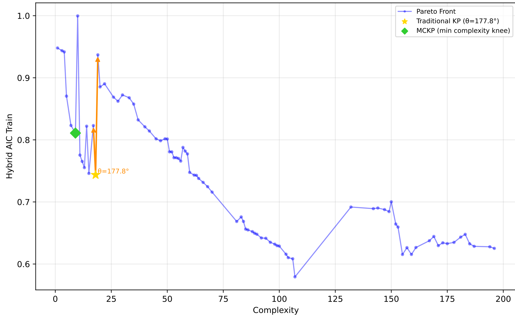
542_pollution - Run 10 - SVP - Hybrid AIC Train \lambda_1=0.00, \lambda_2=0.00, \lambda_3=0.20 | Difficulty: 1.00 | Method: hmr
