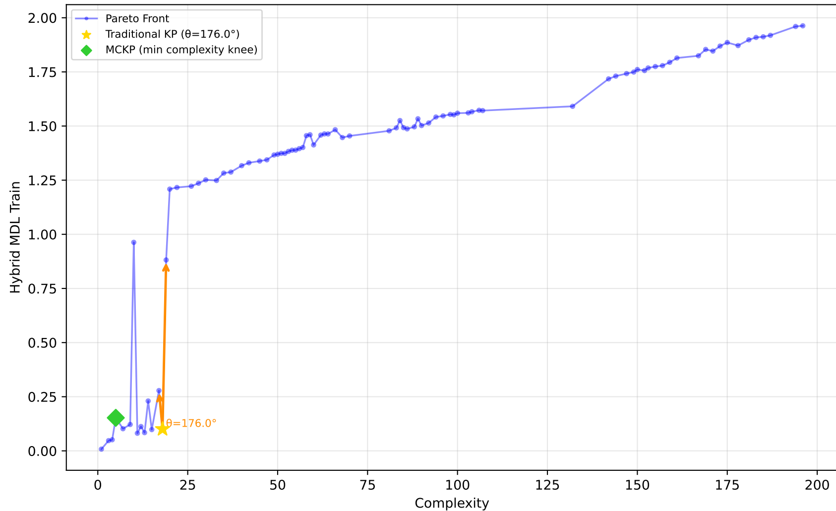
542_pollution - Run 10 - SVP - Hybrid MDL Train \lambda_1=0.70 , \bar{\lambda}_2=1.00 , \lambda_3=0.10 | Difficulty: 1.00 | Method: hmr
