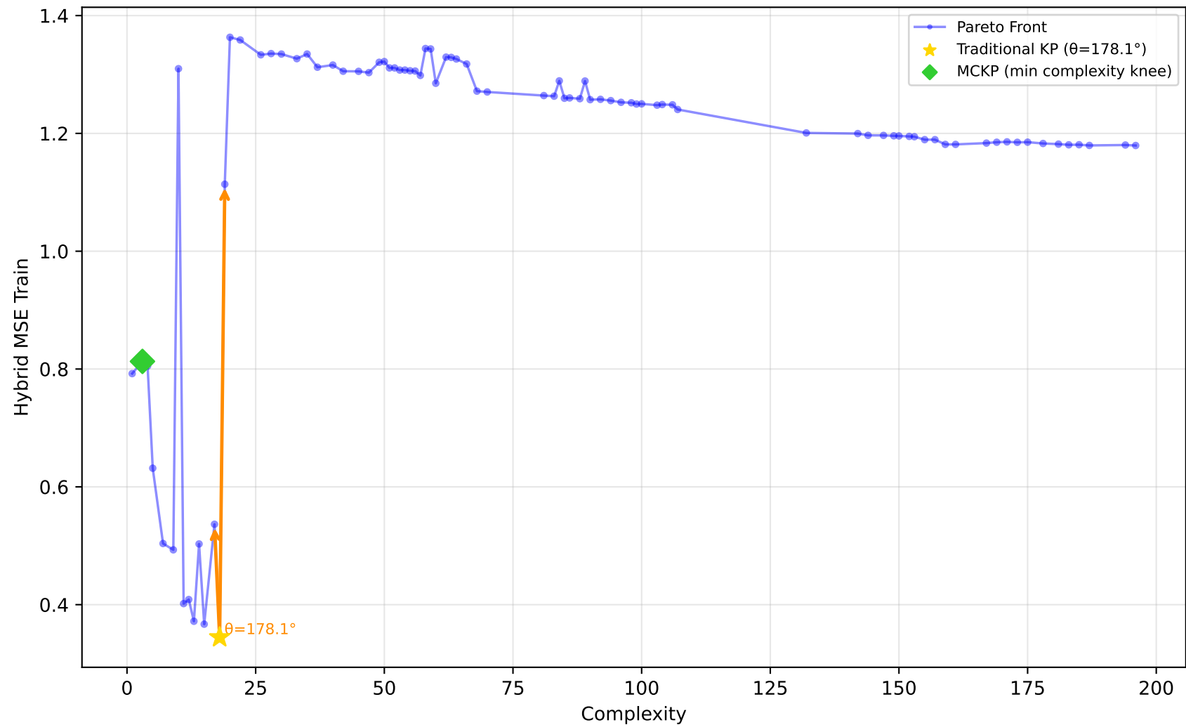
542_pollution - Run 10 - SVP - Hybrid MSE Train \lambda_1=0.70, \lambda_2=1.00, \lambda_3=0.10 | Difficulty: 1.00 | Method: hmr
