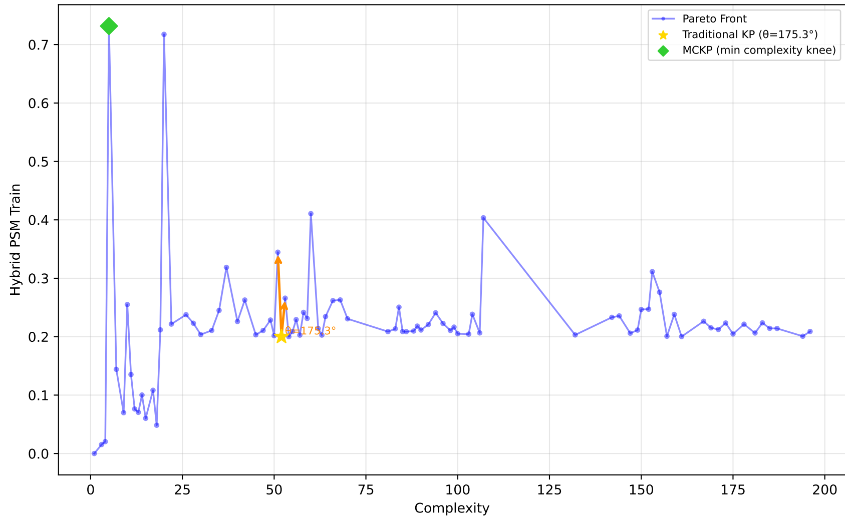
542_pollution - Run 10 - SVP - Hybrid PSM Train \lambda_1=0.00, \lambda_2=0.00, \lambda_3=0.20 | Difficulty: 1.00 | Method: hmr
