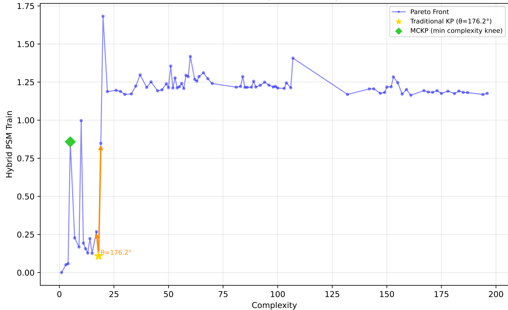
542_pollution - Run 10 - SVP - Hybrid PSM Train \lambda_1=0.70 , \bar{\lambda}_2=1.00 , \lambda_3=0.10 | Difficulty: 1.00 | Method: hmr
