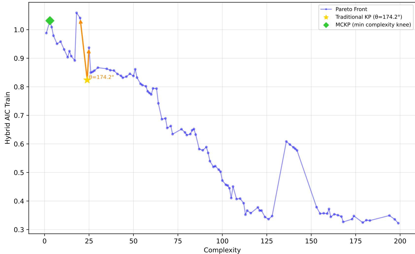
542_pollution - Run 11 - MVP - Hybrid AIC Train \lambda_1=1.00, \lambda_2=0.10, \lambda_3=0.00 | Difficulty: 0.14 | Method: mckp
