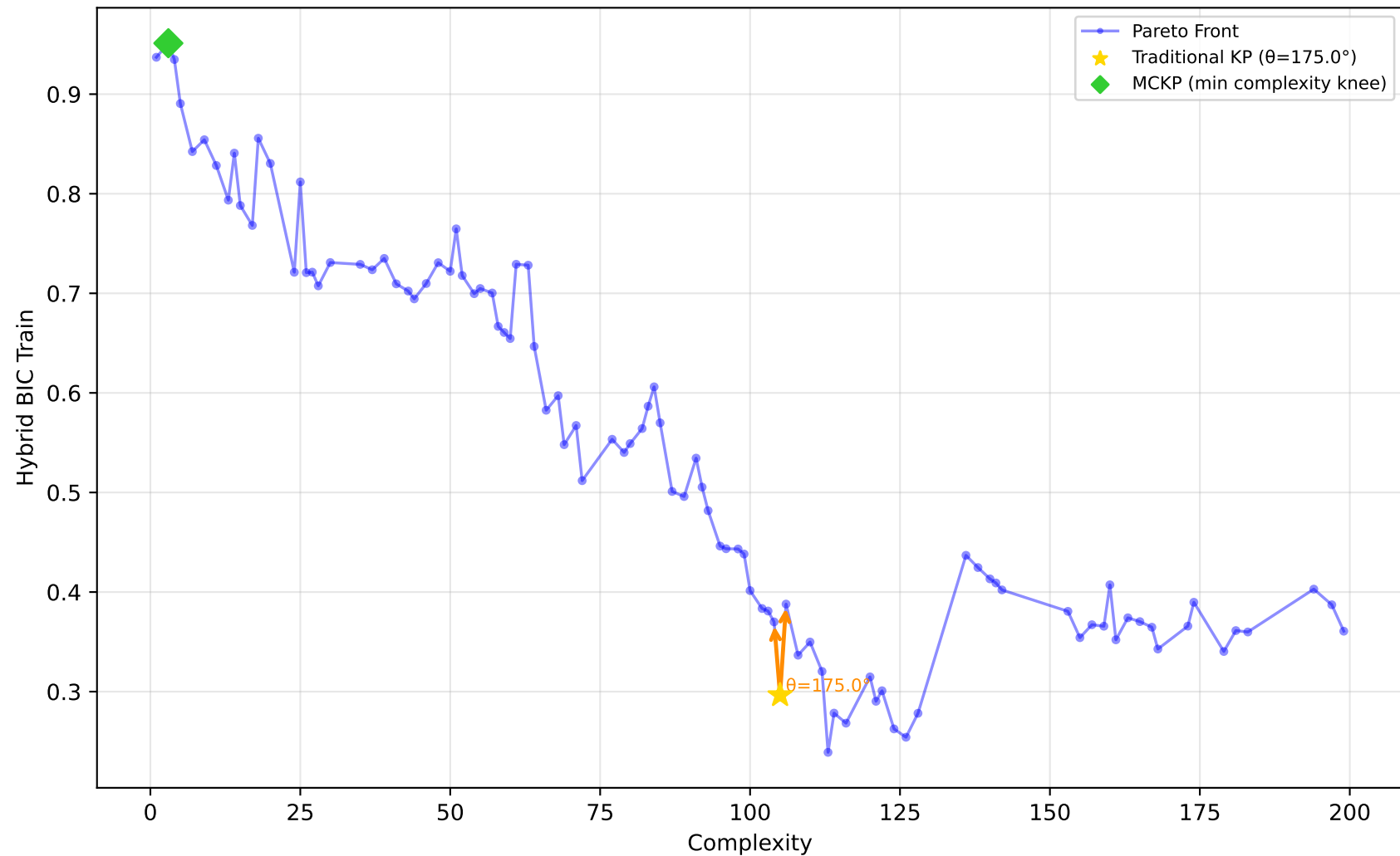
542_pollution - Run 11 - MVP - Hybrid BIC Train \lambda_1=0.40, \lambda_2=0.10, \lambda_3=0.00 | Difficulty: 0.14 | Method: mckp
