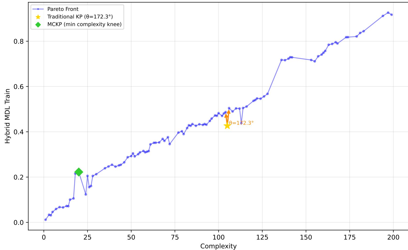
542_pollution - Run 11 - MVP - Hybrid MDL Train \lambda_1=0.40, \lambda_2=0.10, \lambda_3=0.00 | Difficulty: 0.14 | Method: mckp
