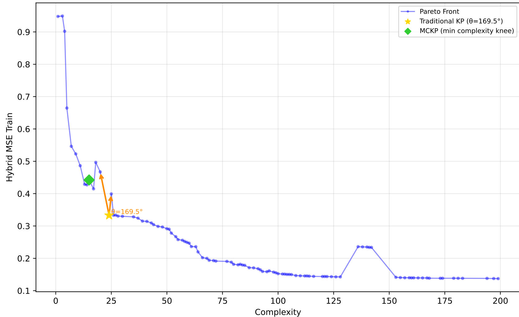
542_pollution - Run 11 - MVP - Hybrid MSE Train \lambda_1=0.40, \lambda_2=0.10, \lambda_3=0.00 | Difficulty: 0.14 | Method: mckp
