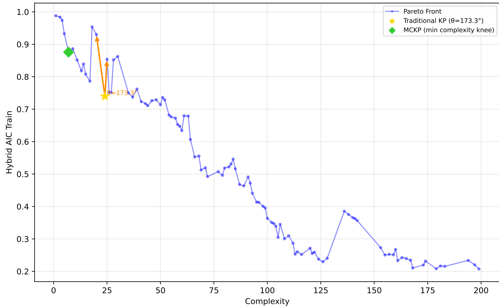
542_pollution - Run 11 - SVP - Hybrid AIC Train \lambda_1=0.00, \lambda_2=0.00, \lambda_3=0.20 | Difficulty: 0.14 | Method: mckp
