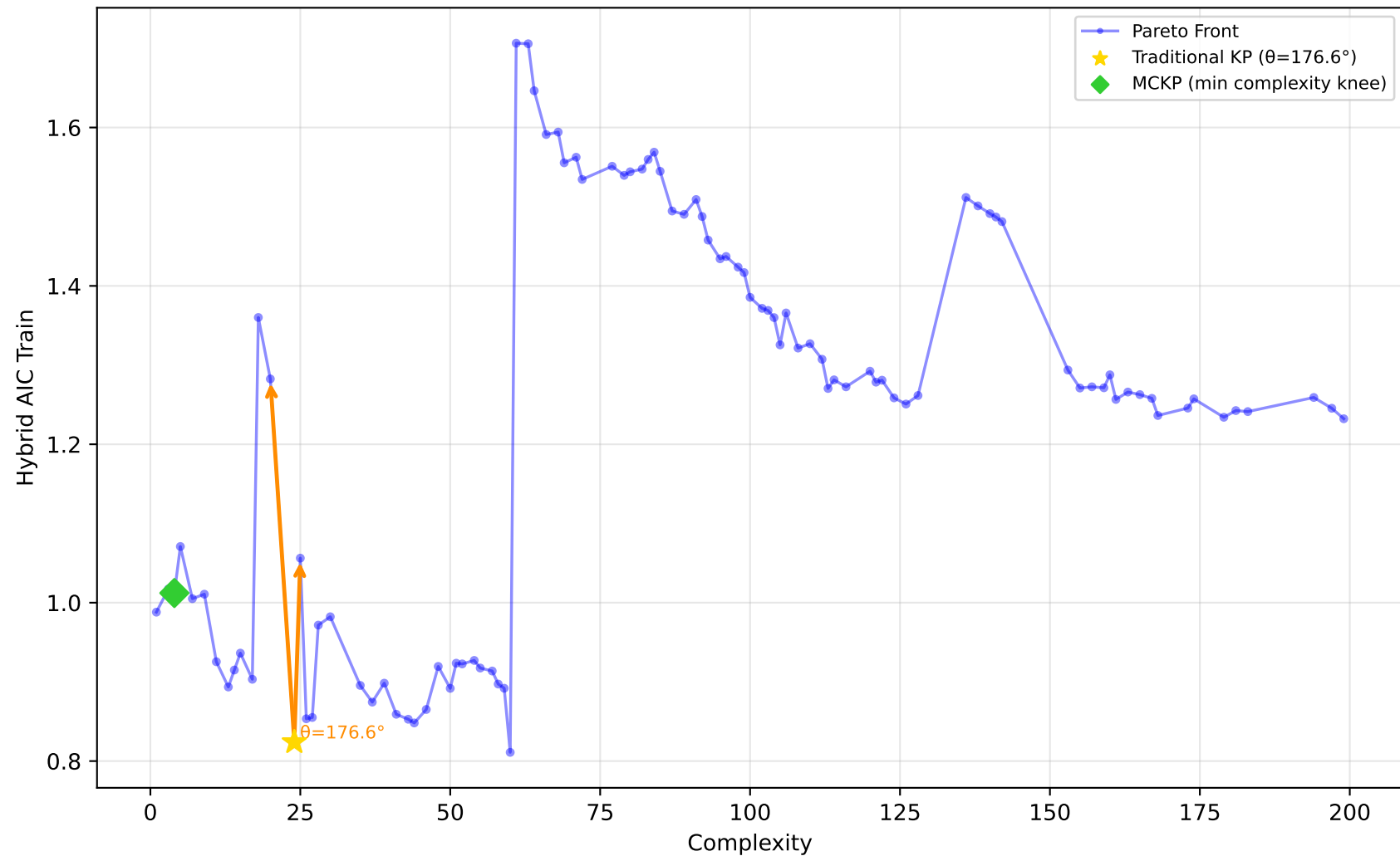
542_pollution - Run 11 - SVP - Hybrid AIC Train \lambda_1=0.70 , \lambda_2=1.00 , \lambda_3=0.10 | Difficulty: 0.14 | Method: mckp
