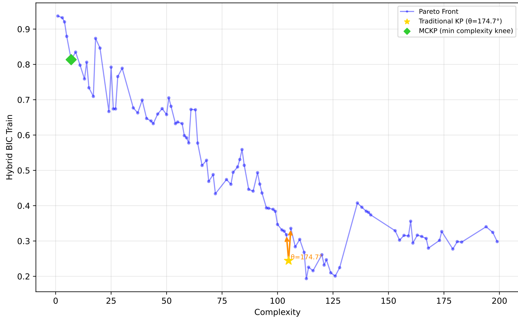
542_pollution - Run 11 - SVP - Hybrid BIC Train \lambda_1=0.00, \lambda_2=0.00, \lambda_3=0.20 | Difficulty: 0.14 | Method: mckp
