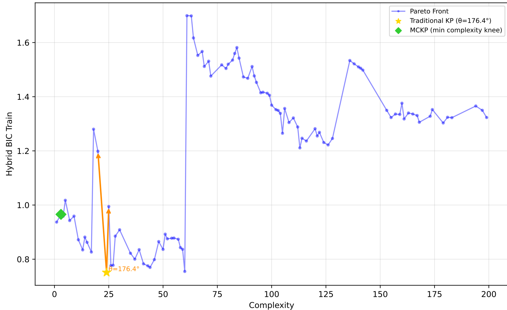
542_pollution - Run 11 - SVP - Hybrid BIC Train \lambda_1=0.70 , \lambda_2=1.00 , \lambda_3=0.10 | Difficulty: 0.14 | Method: mckp
