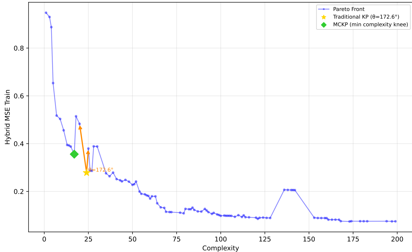
542_pollution - Run 11 - SVP - Hybrid MSE Train \lambda_1=0.00, \lambda_2=0.00, \lambda_3=0.20 | Difficulty: 0.14 | Method: mckp
