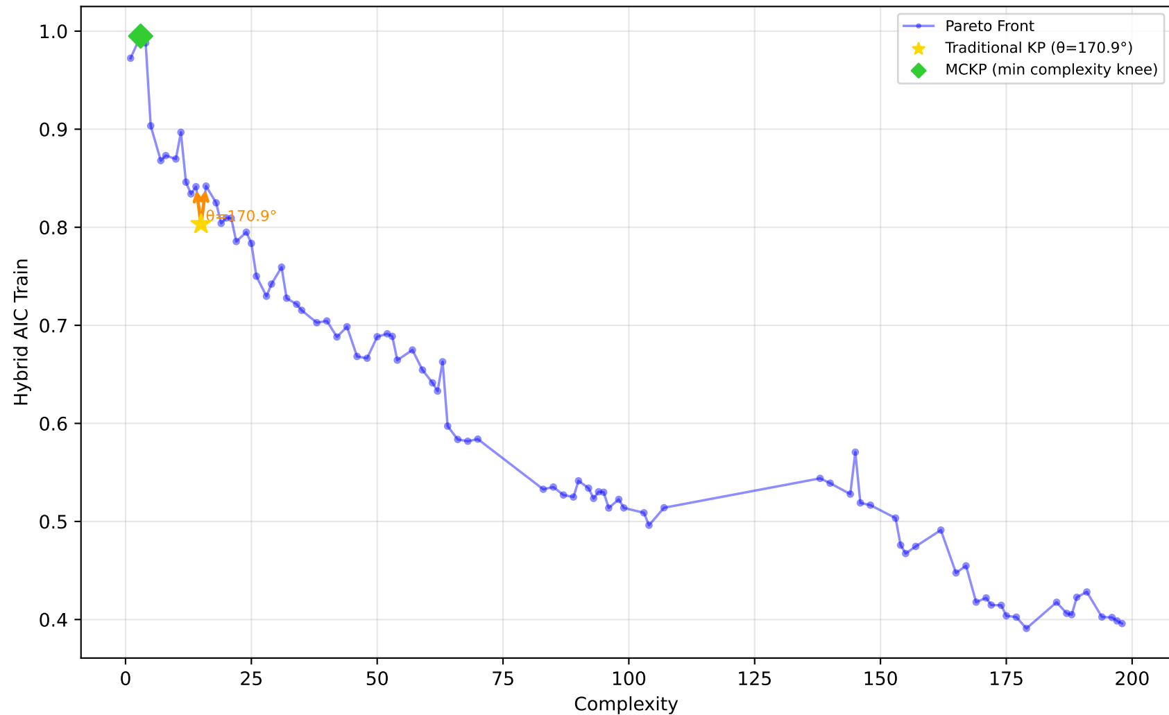
542_pollution - Run 12 - MVP - Hybrid AIC Train \lambda_1=0.40 , \lambda_2=0.10 , \lambda_3=0.00 | Difficulty: 0.77 | Method: hmr
