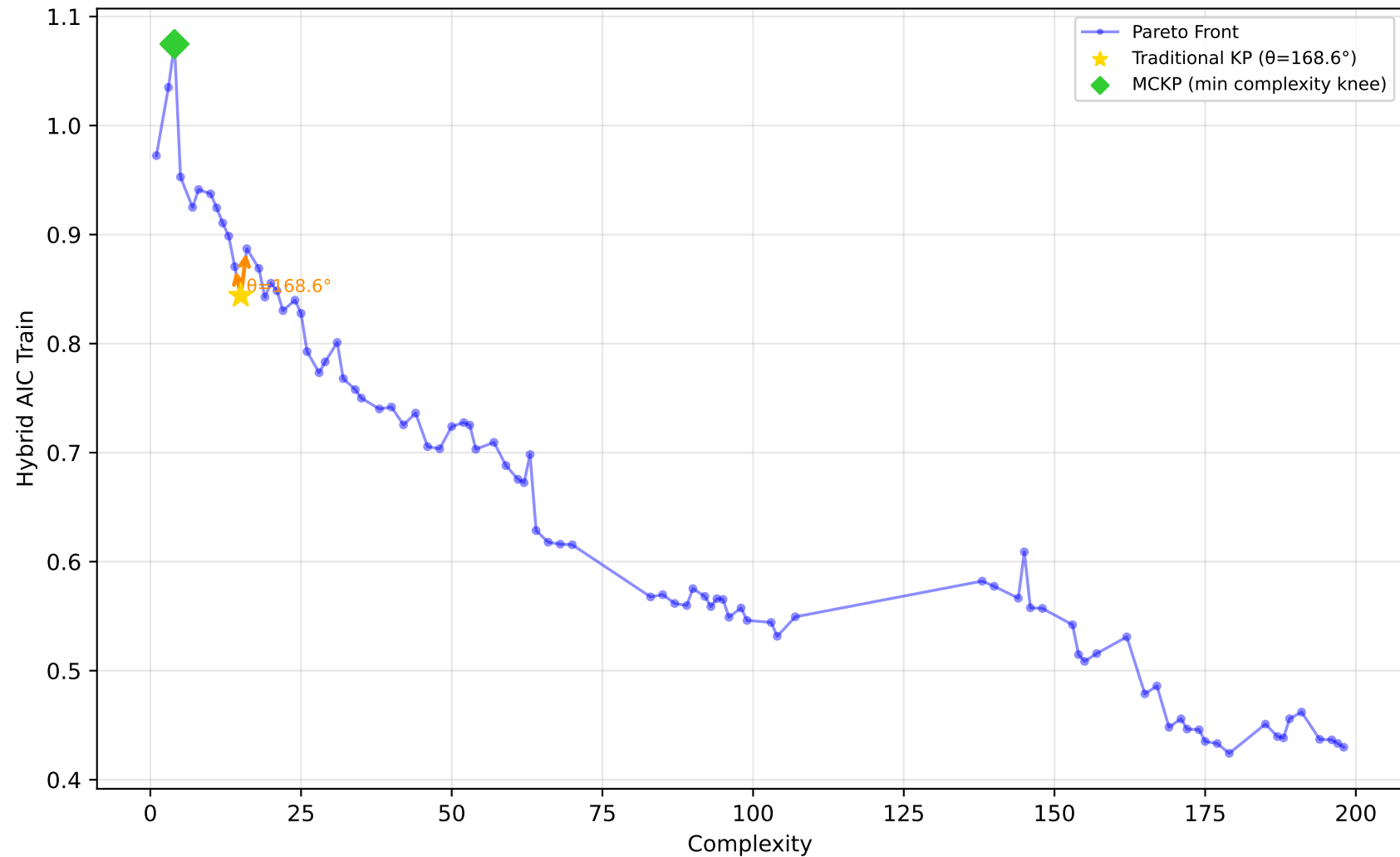
542_pollution - Run 12 - MVP - Hybrid AIC Train \lambda_1=1.00, \bar{\lambda}_2=0.10, \lambda_3=0.00 | Difficulty: 0.77 | Method: hmr
