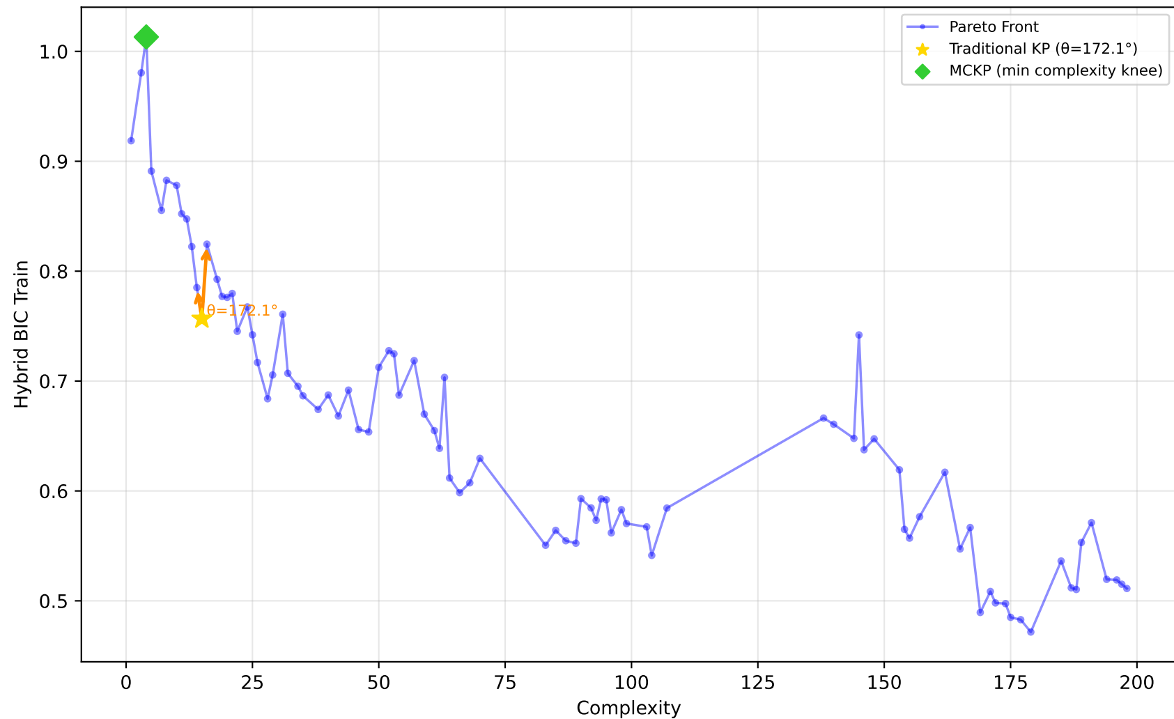
542_pollution - Run 12 - MVP - Hybrid BIC Train \lambda_1=1.00 , \lambda_2=0.10 , \lambda_3=0.00 | Difficulty: 0.77 | Method: hmr
