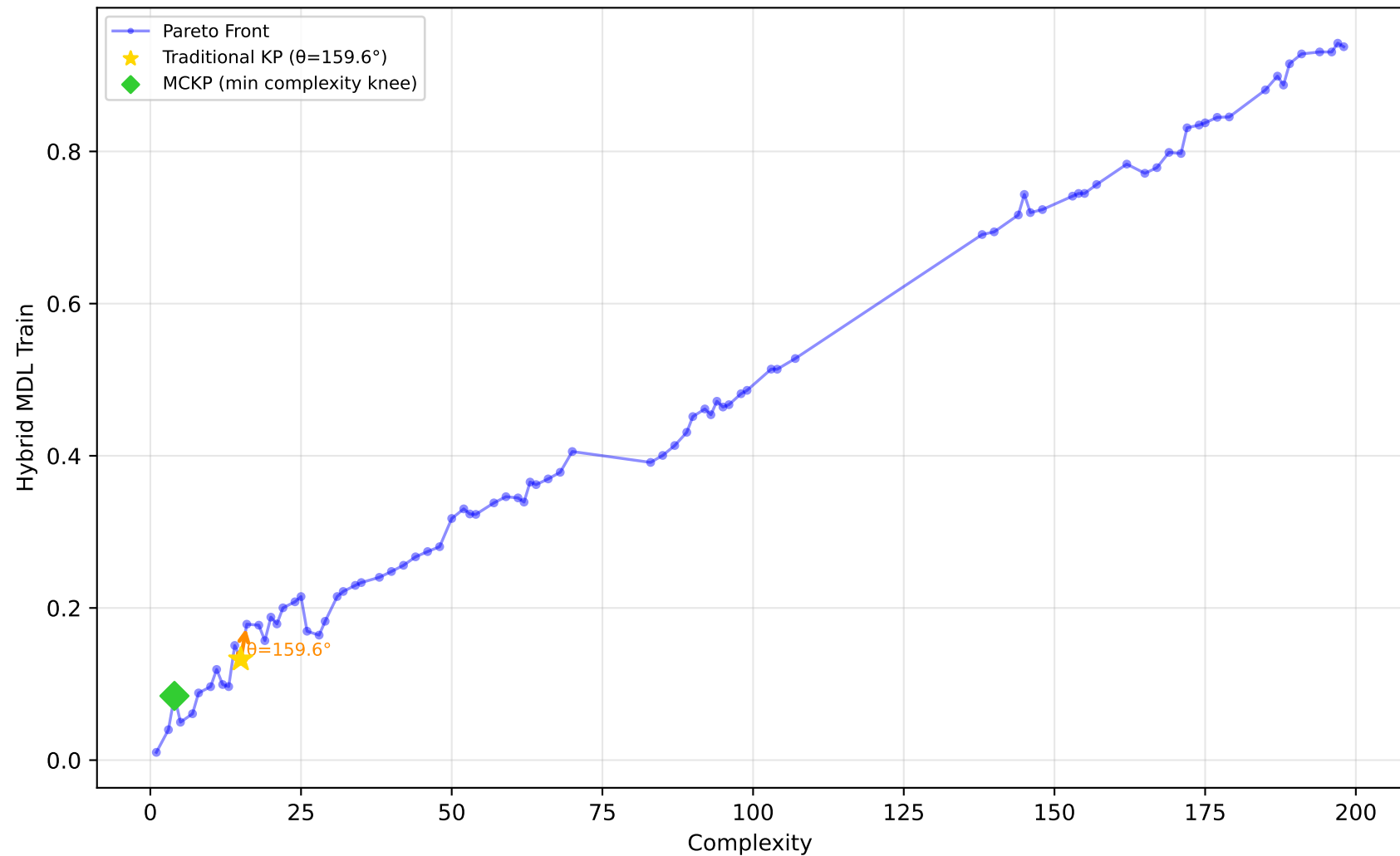
542_pollution - Run 12 - MVP - Hybrid MDL Train \lambda_1=0.40, \lambda_2=0.10, \lambda_3=0.00 | Difficulty: 0.77 | Method: hmr
