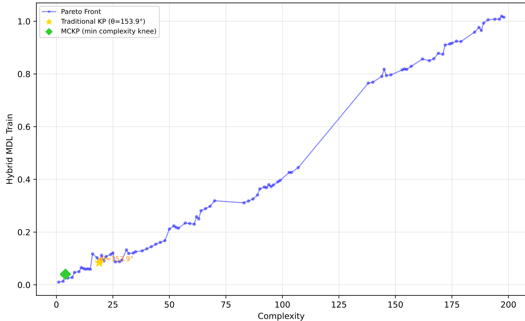
542_pollution - Run 12 - SVP - Hybrid MDL Train \lambda_1=0.00, \lambda_2=0.00, \lambda_3=0.20 | Difficulty: 0.77 | Method: hmr
