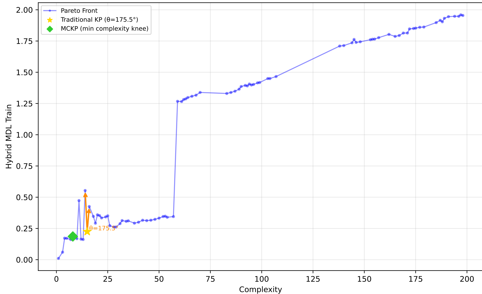
542_pollution - Run 12 - SVP - Hybrid MDL Train \lambda_1=0.70, \bar{\lambda}_2=1.00, \lambda_3=0.10 | Difficulty: 0.77 | Method: hmr
