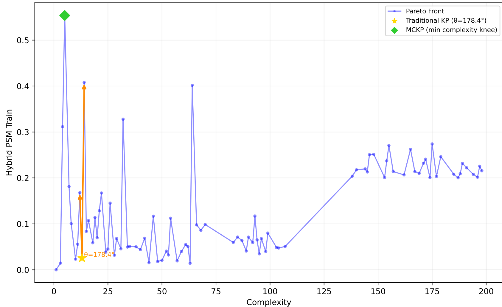
542_pollution - Run 12 - SVP - Hybrid PSM Train \lambda_1=0.00, \lambda_2=0.00, \lambda_3=0.20 | Difficulty: 0.77 | Method: hmr
