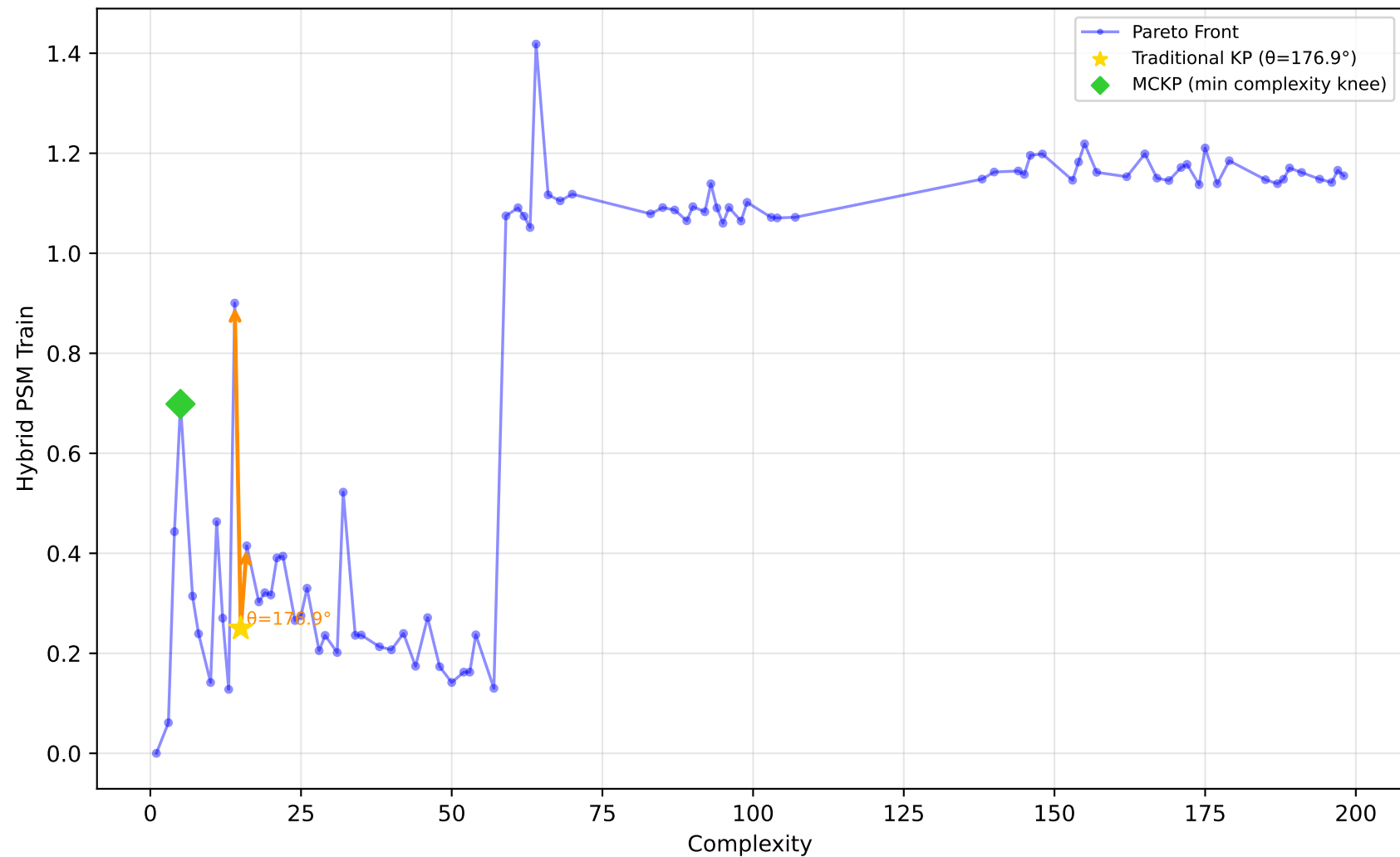
542_pollution - Run 12 - SVP - Hybrid PSM Train \lambda_1=0.70 , \lambda_2=1.00 , \lambda_3=0.10 | Difficulty: 0.77 | Method: hmr
