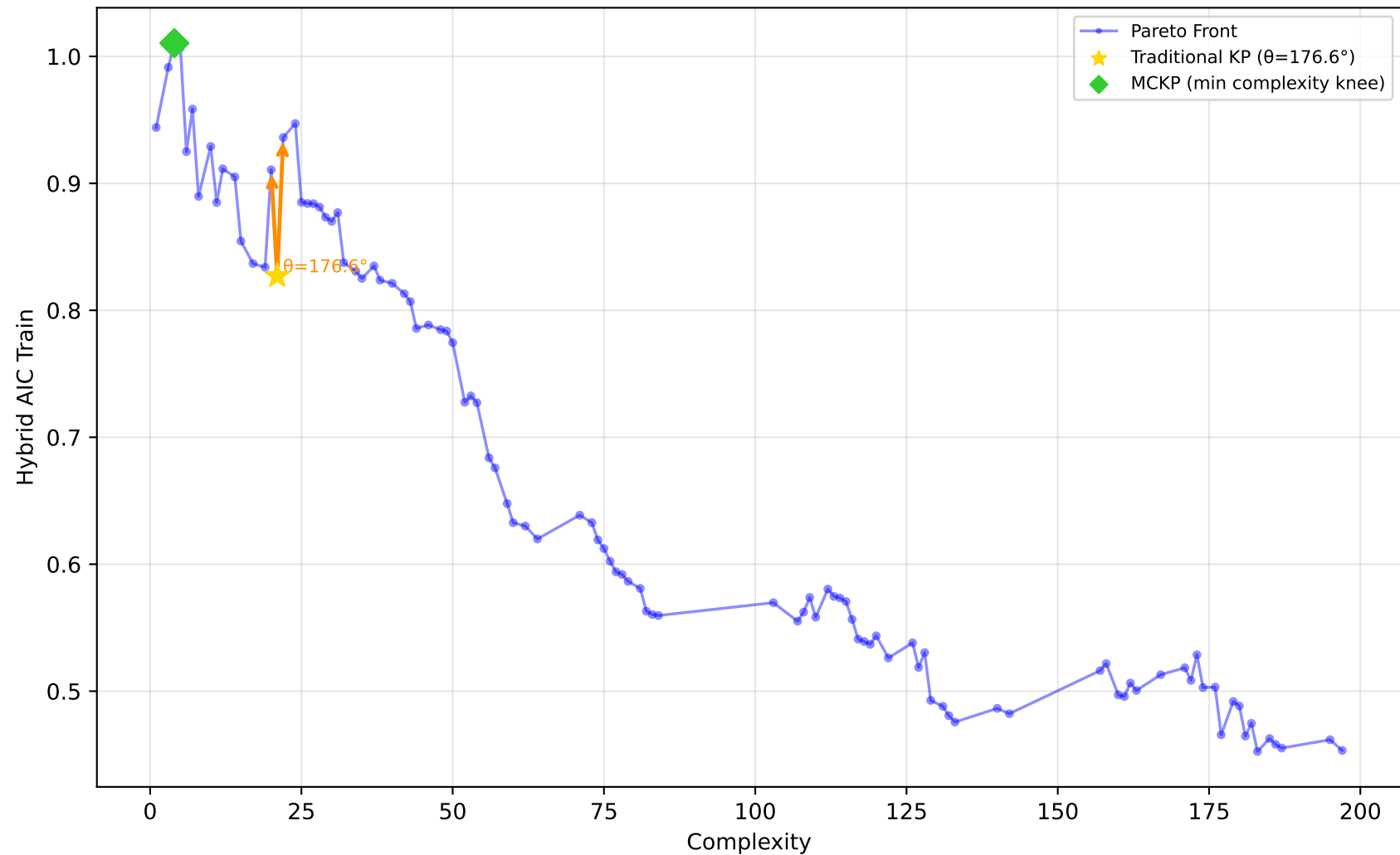
542_pollution - Run 13 - MVP - Hybrid AIC Train \lambda_1=1.00, \lambda_2=0.10, \lambda_3=0.00 | Difficulty: 0.22 | Method: mckp
