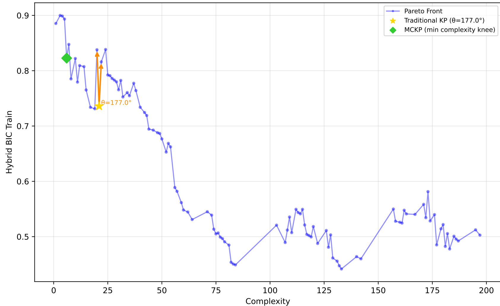
542_pollution - Run 13 - MVP - Hybrid BIC Train \lambda_1=0.40, \lambda_2=0.10, \lambda_3=0.00 | Difficulty: 0.22 | Method: mckp
