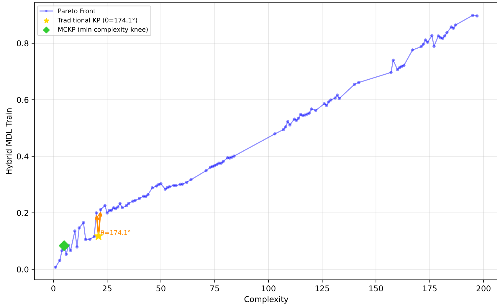
542_pollution - Run 13 - MVP - Hybrid MDL Train \lambda_1=0.40, \lambda_2=0.10, \lambda_3=0.00 | Difficulty: 0.22 | Method: mckp
