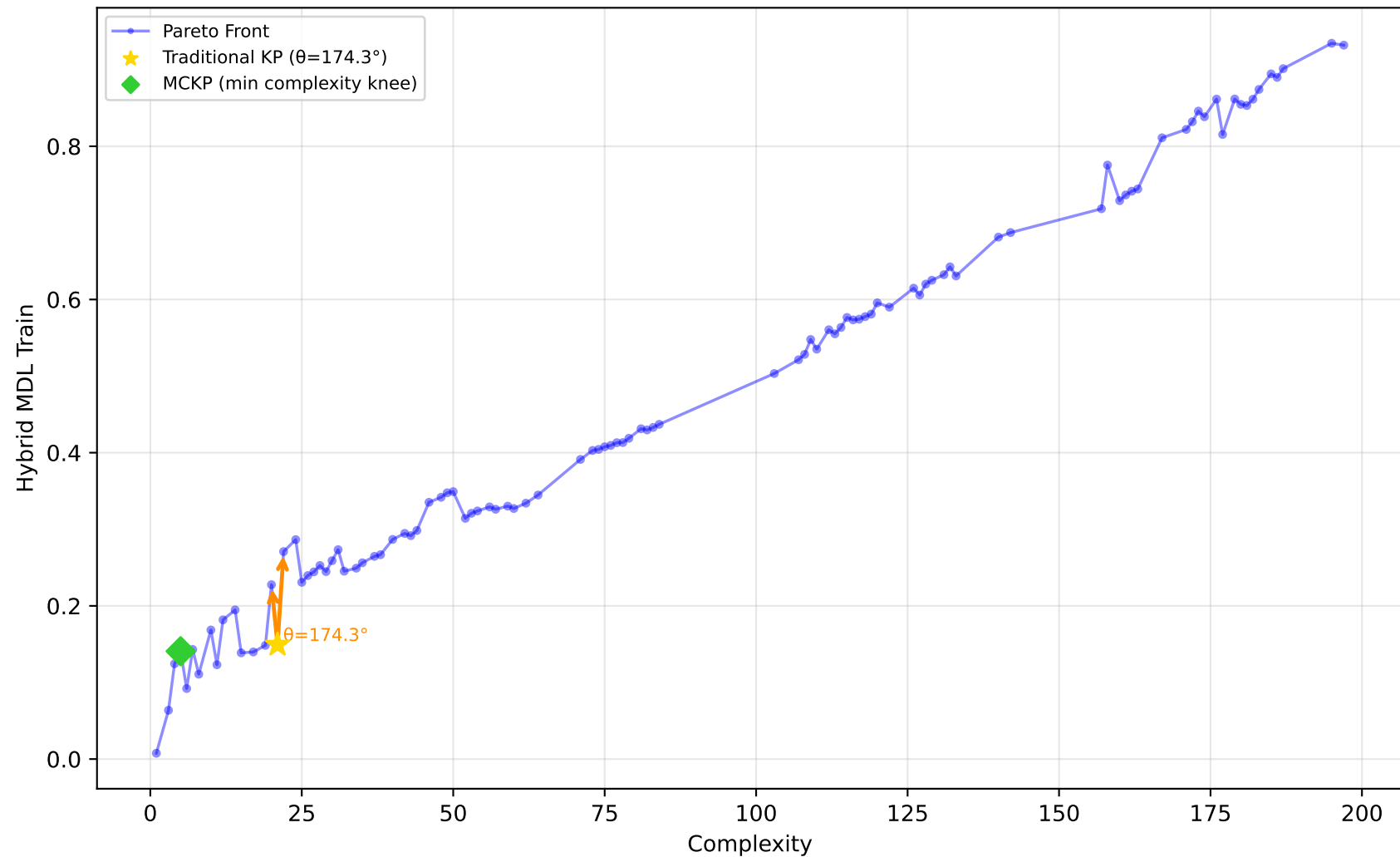
542_pollution - Run 13 - MVP - Hybrid MDL Train \lambda_1=1.00, \bar{\lambda}_2=0.10, \lambda_3=0.00 | Difficulty: 0.22 | Method: mckp
