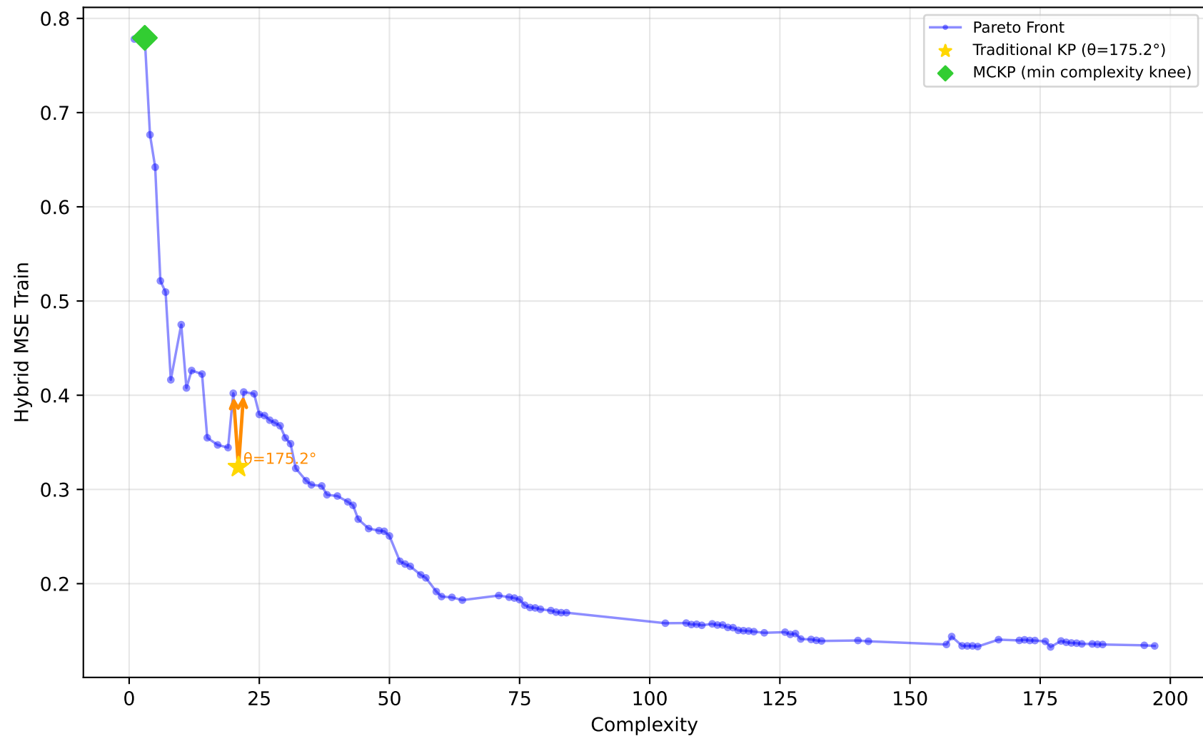
542_pollution - Run 13 - MVP - Hybrid MSE Train \lambda_1=0.40, \lambda_2=0.10, \lambda_3=0.00 | Difficulty: 0.22 | Method: mckp
