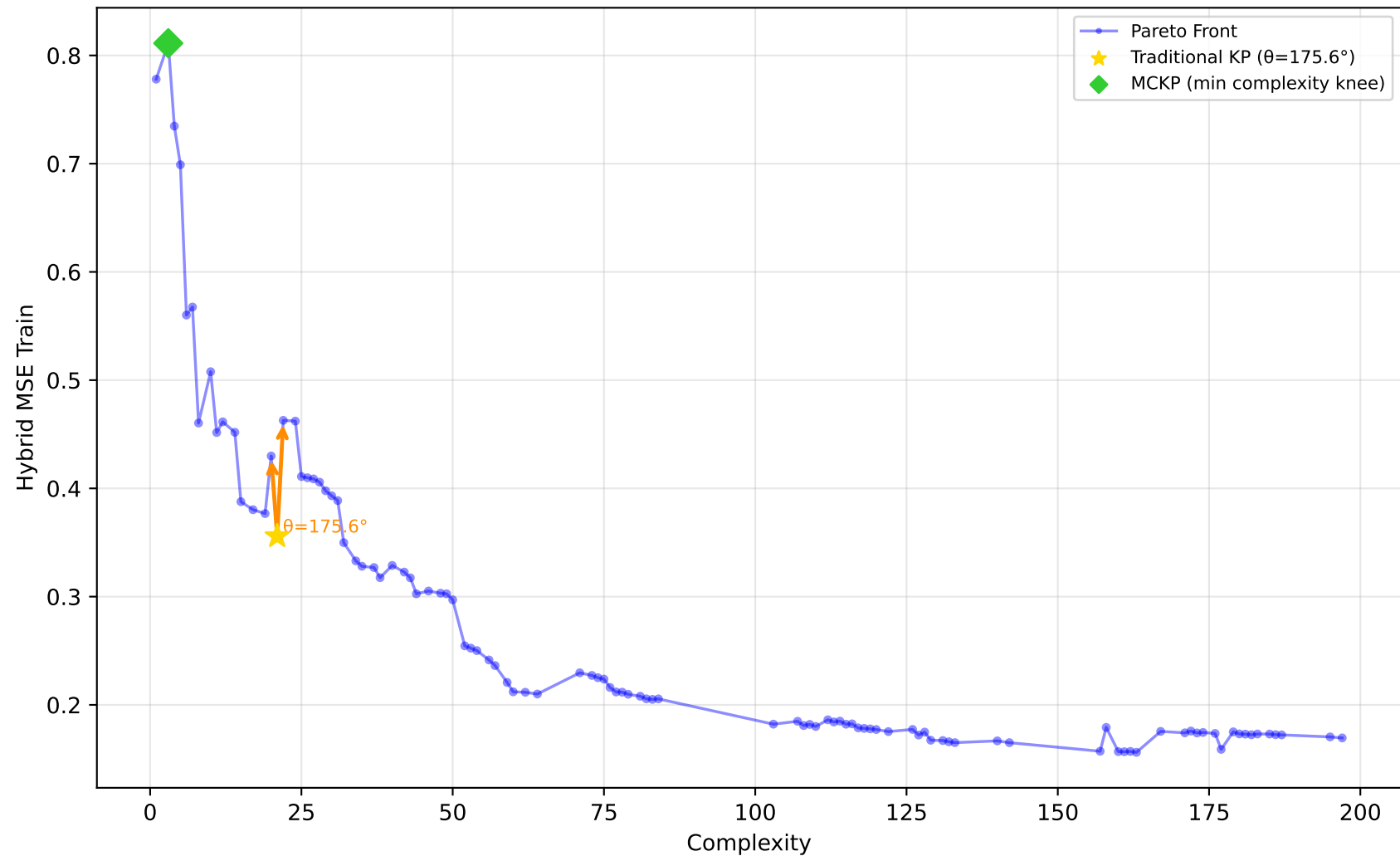
542_pollution - Run 13 - MVP - Hybrid MSE Train \lambda_1=1.00, \bar{\lambda}_2=0.10, \lambda_3=0.00 | Difficulty: 0.22 | Method: mckp
