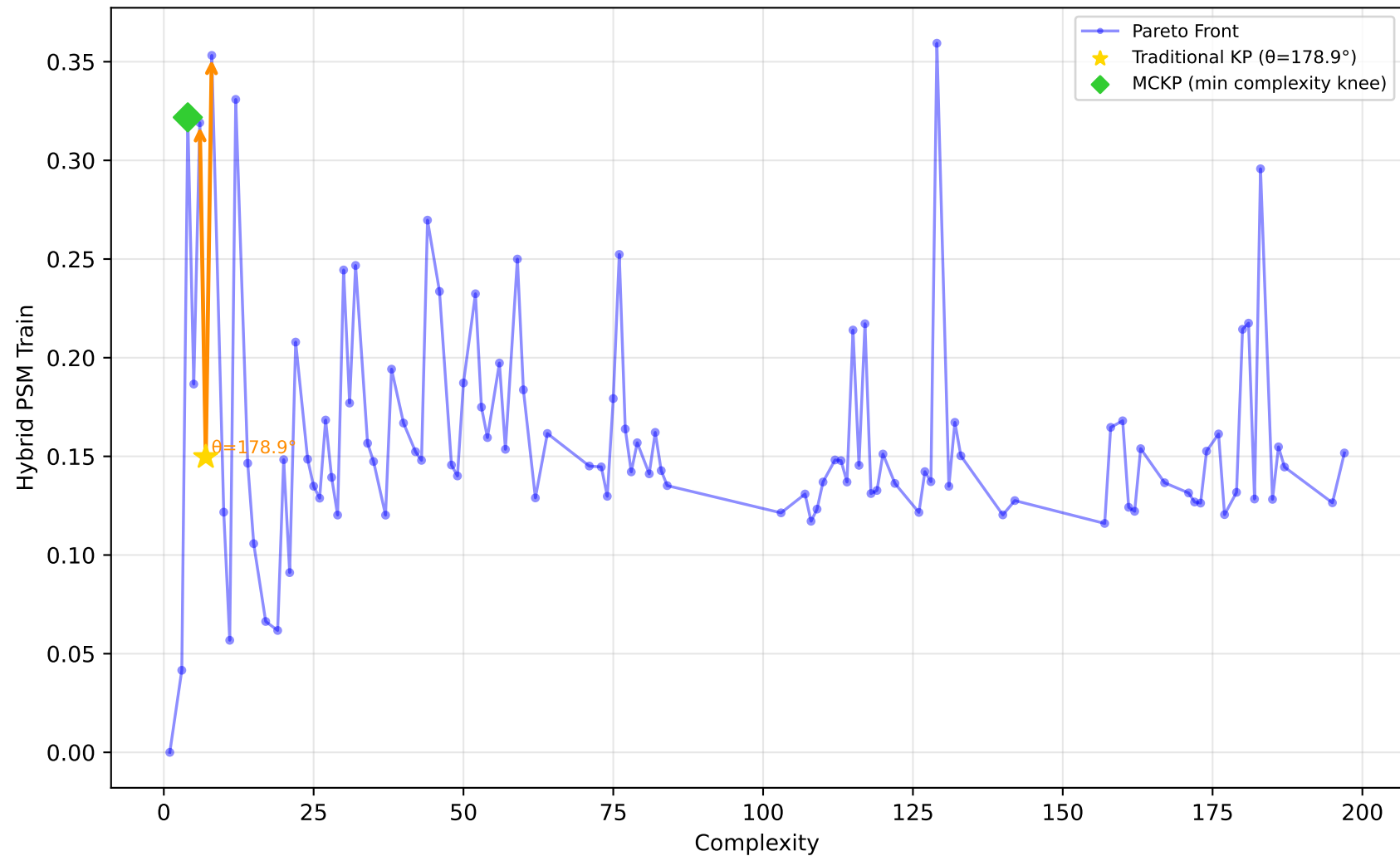
542_pollution - Run 13 - MVP - Hybrid PSM Train \lambda_1=0.40, \lambda_2=0.10, \lambda_3=0.00 | Difficulty: 0.22 | Method: mckp
