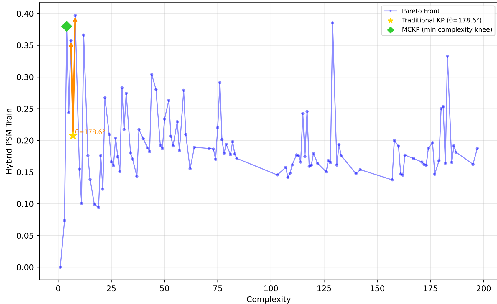
542_pollution - Run 13 - MVP - Hybrid PSM Train \lambda_1=1.00, \lambda_2=0.10, \lambda_3=0.00 | Difficulty: 0.22 | Method: mckp
