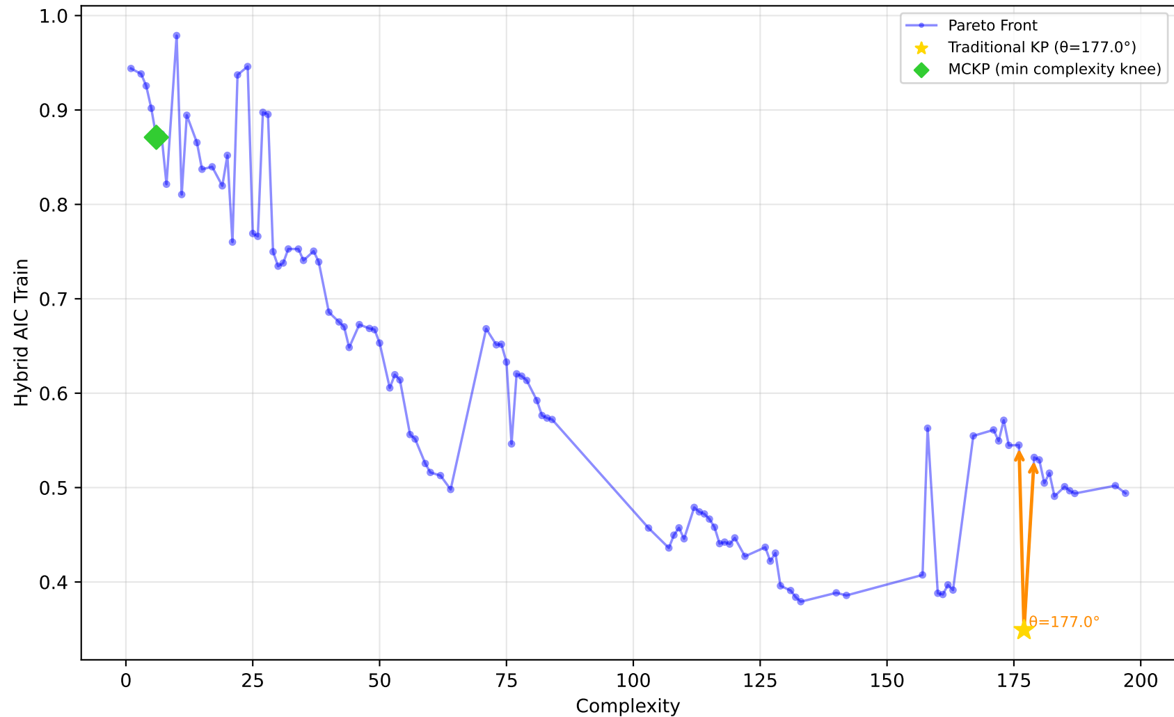
542_pollution - Run 13 - SVP - Hybrid AIC Train \lambda_1=0.00, \lambda_2=0.00, \lambda_3=0.20 | Difficulty: 0.22 | Method: mckp
