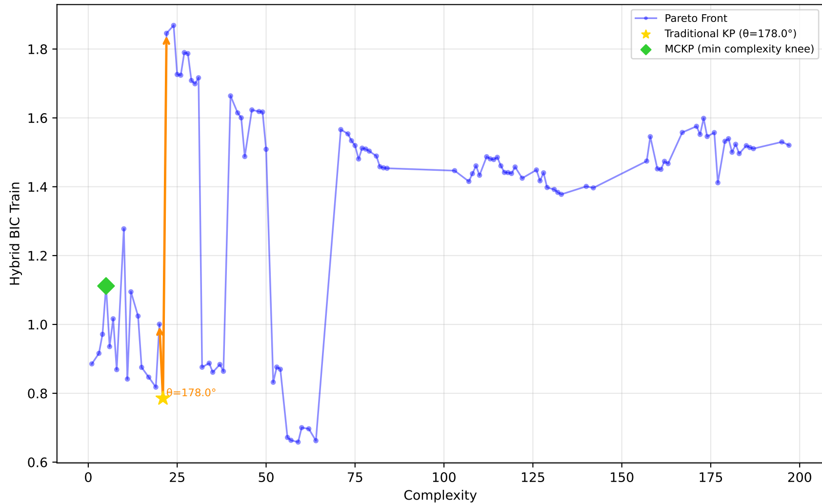
542_pollution - Run 13 - SVP - Hybrid BIC Train \lambda_1=0.70, \lambda_2=1.00, \lambda_3=0.10 | Difficulty: 0.22 | Method: mckp
