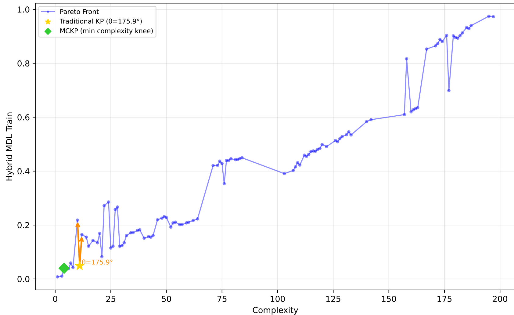
542_pollution - Run 13 - SVP - Hybrid MDL Train \lambda_1=0.00, \lambda_2=0.00, \lambda_3=0.20 | Difficulty: 0.22 | Method: mckp
