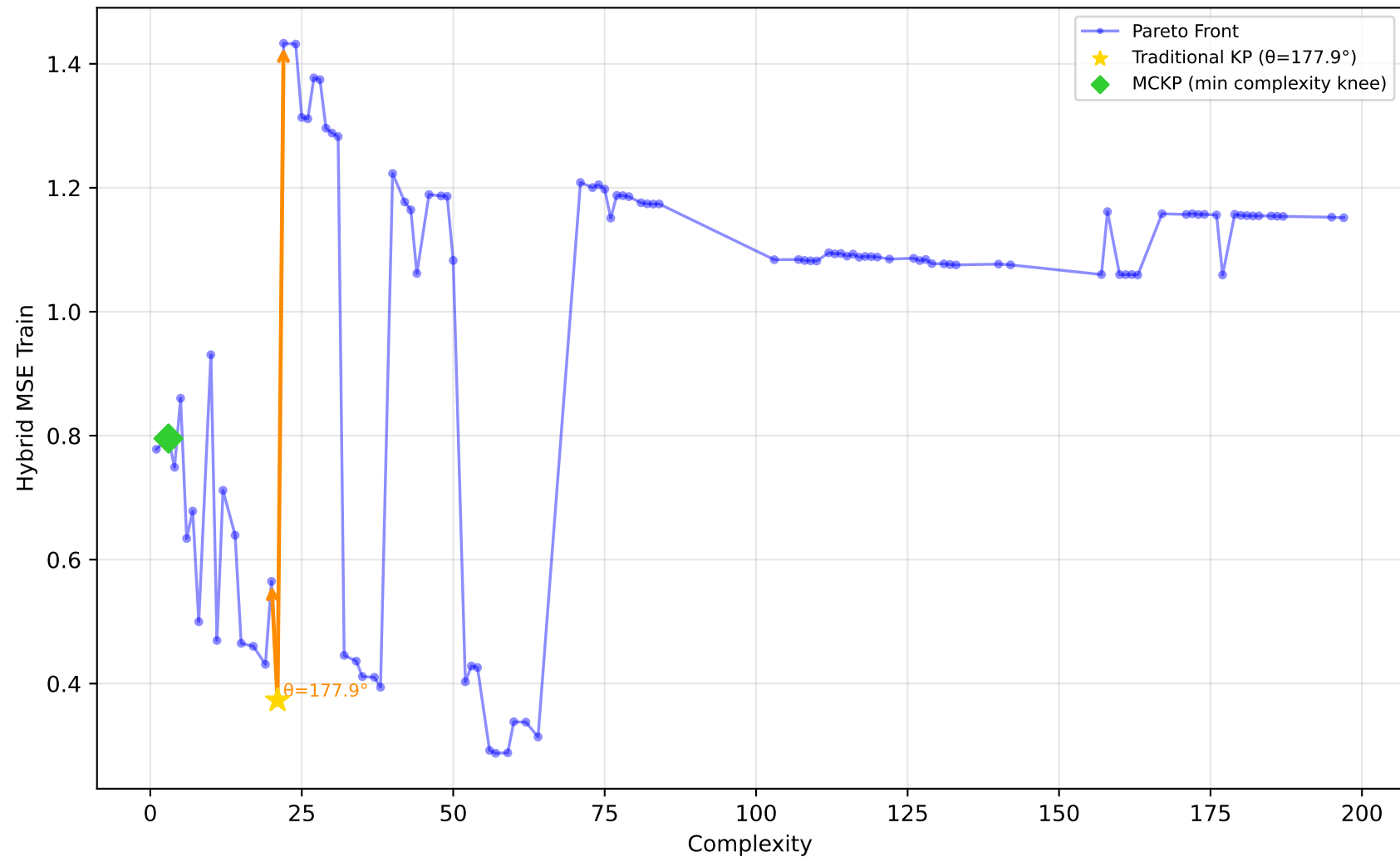
542_pollution - Run 13 - SVP - Hybrid MSE Train \lambda_1=0.70, \lambda_2=1.00, \lambda_3=0.10 | Difficulty: 0.22 | Method: mckp
