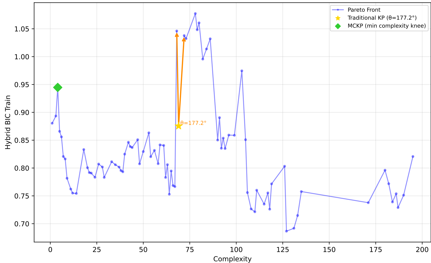
542_pollution - Run 14 - MVP - Hybrid BIC Train \lambda_1=0.40, \lambda_2=0.10, \lambda_3=0.00 | Difficulty: 1.00 | Method: hmr
