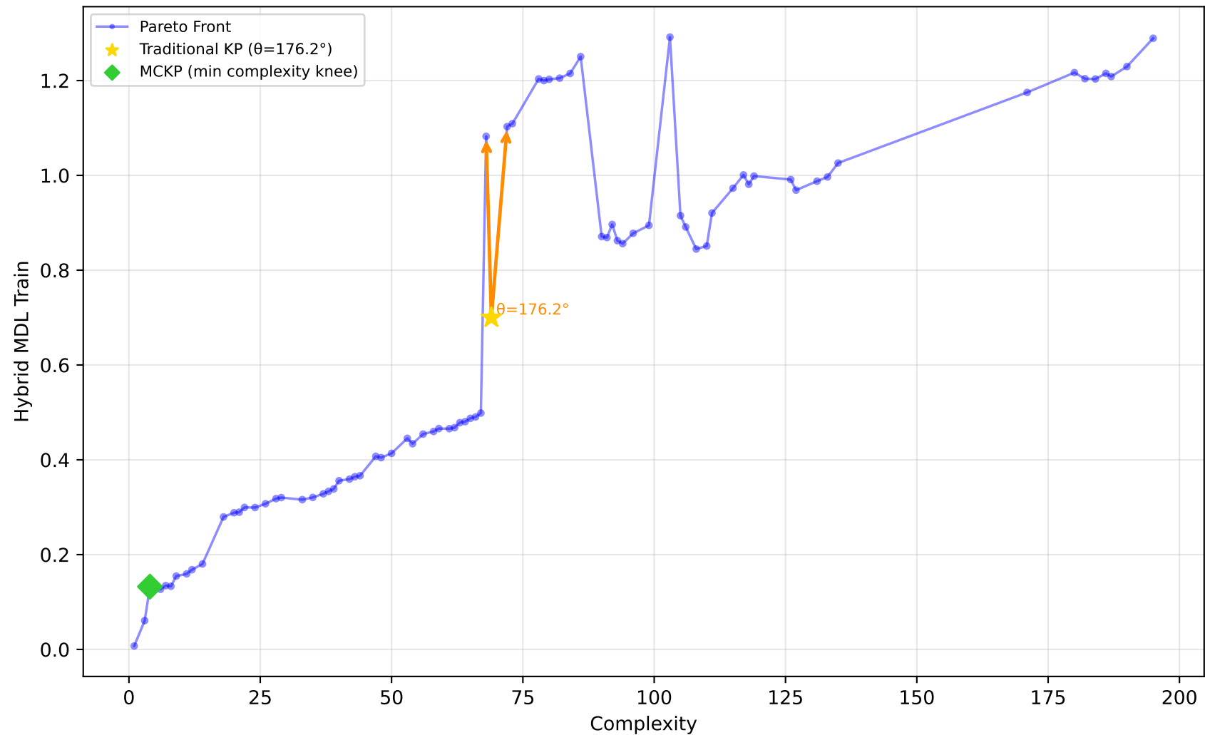
542_pollution - Run 14 - MVP - Hybrid MDL Train \lambda_1=1.00, \lambda_2=0.10, \lambda_3=0.00 | Difficulty: 1.00 | Method: hmr
