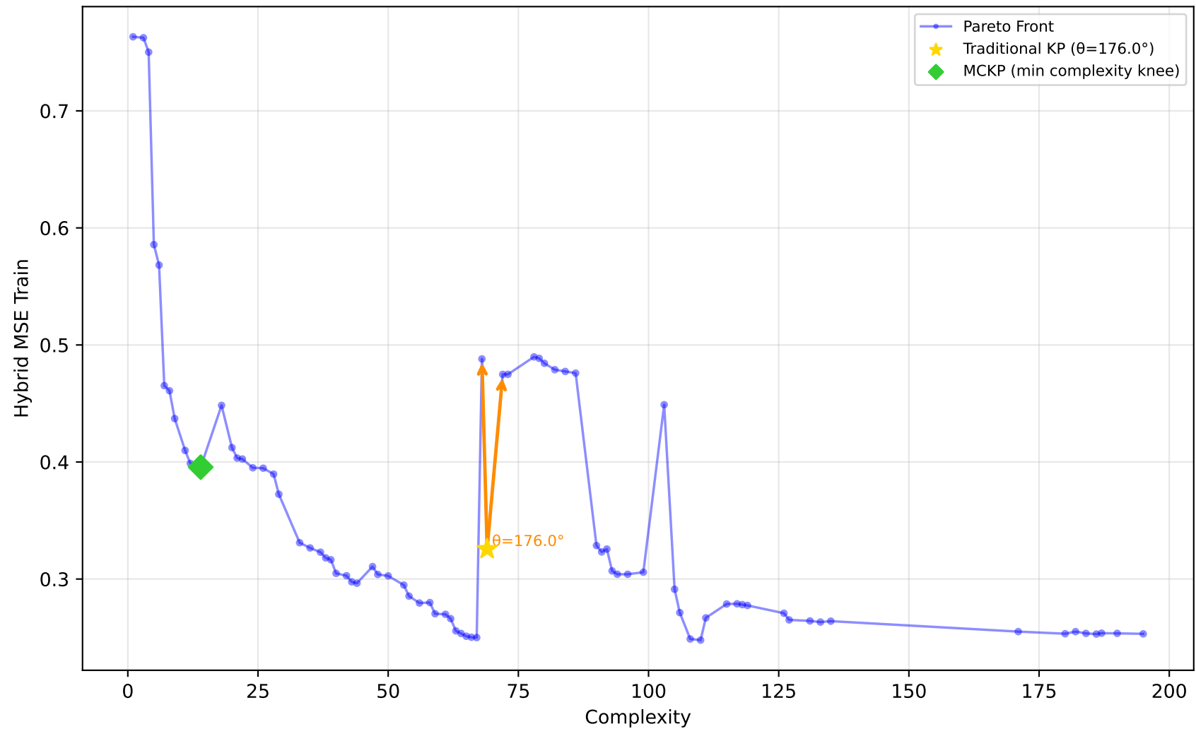
542_pollution - Run 14 - MVP - Hybrid MSE Train \lambda_1=0.40, \lambda_2=0.10, \lambda_3=0.00 | Difficulty: 1.00 | Method: hmr
