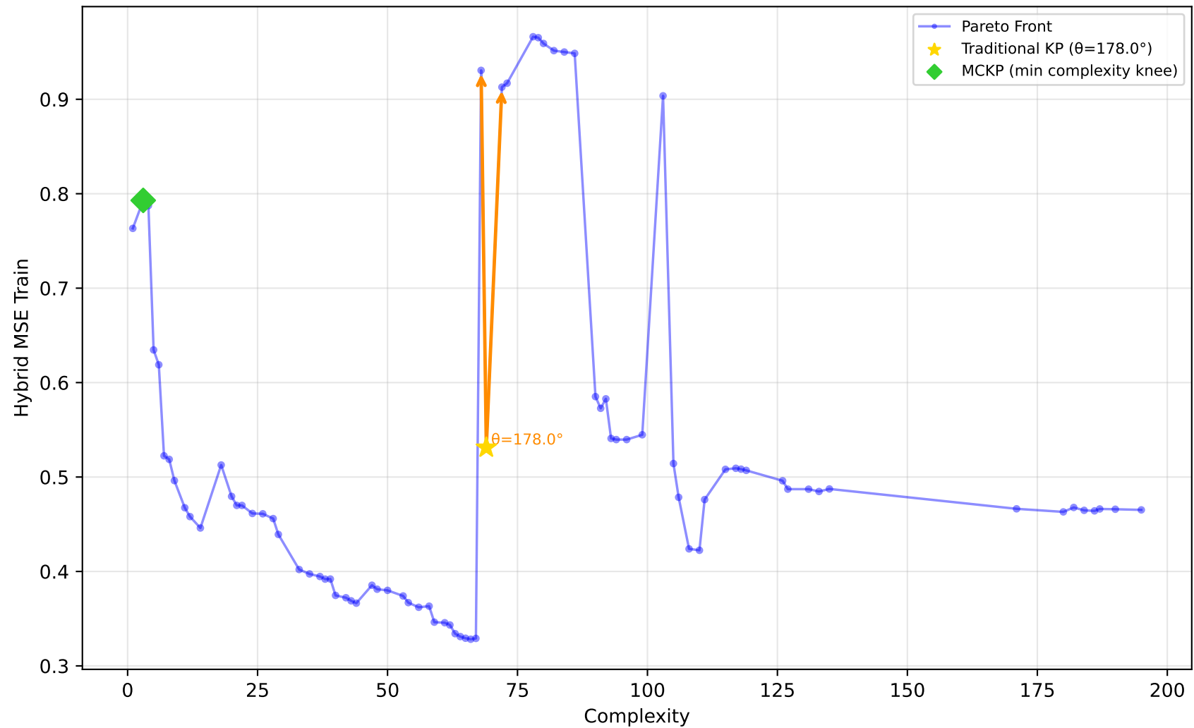
542_pollution - Run 14 - MVP - Hybrid MSE Train \lambda_1=1.00, \lambda_2=0.10, \lambda_3=0.00 | Difficulty: 1.00 | Method: hmr
