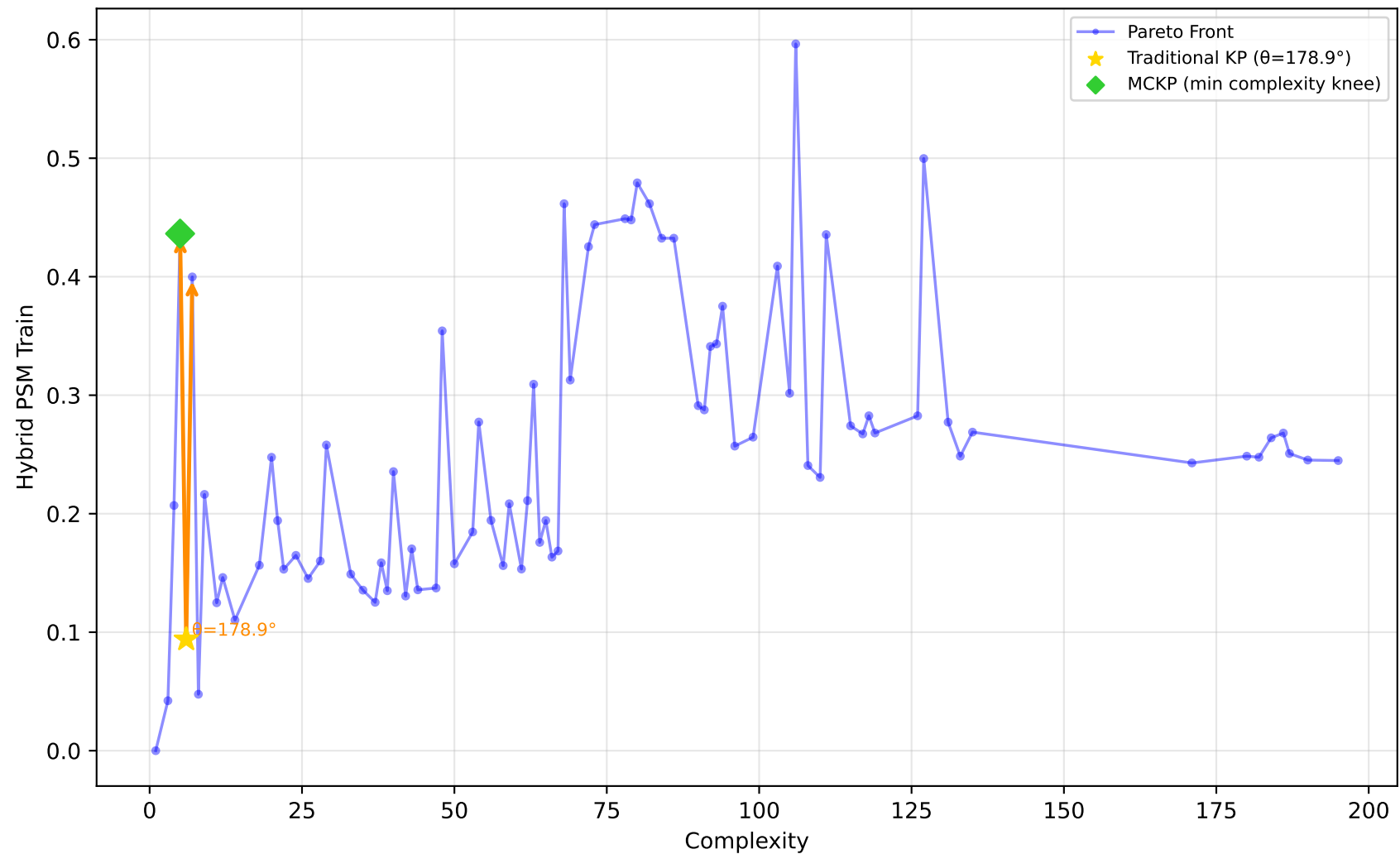
542_pollution - Run 14 - MVP - Hybrid PSM Train \lambda_1=0.40, \lambda_2=0.10, \lambda_3=0.00 | Difficulty: 1.00 | Method: hmr
