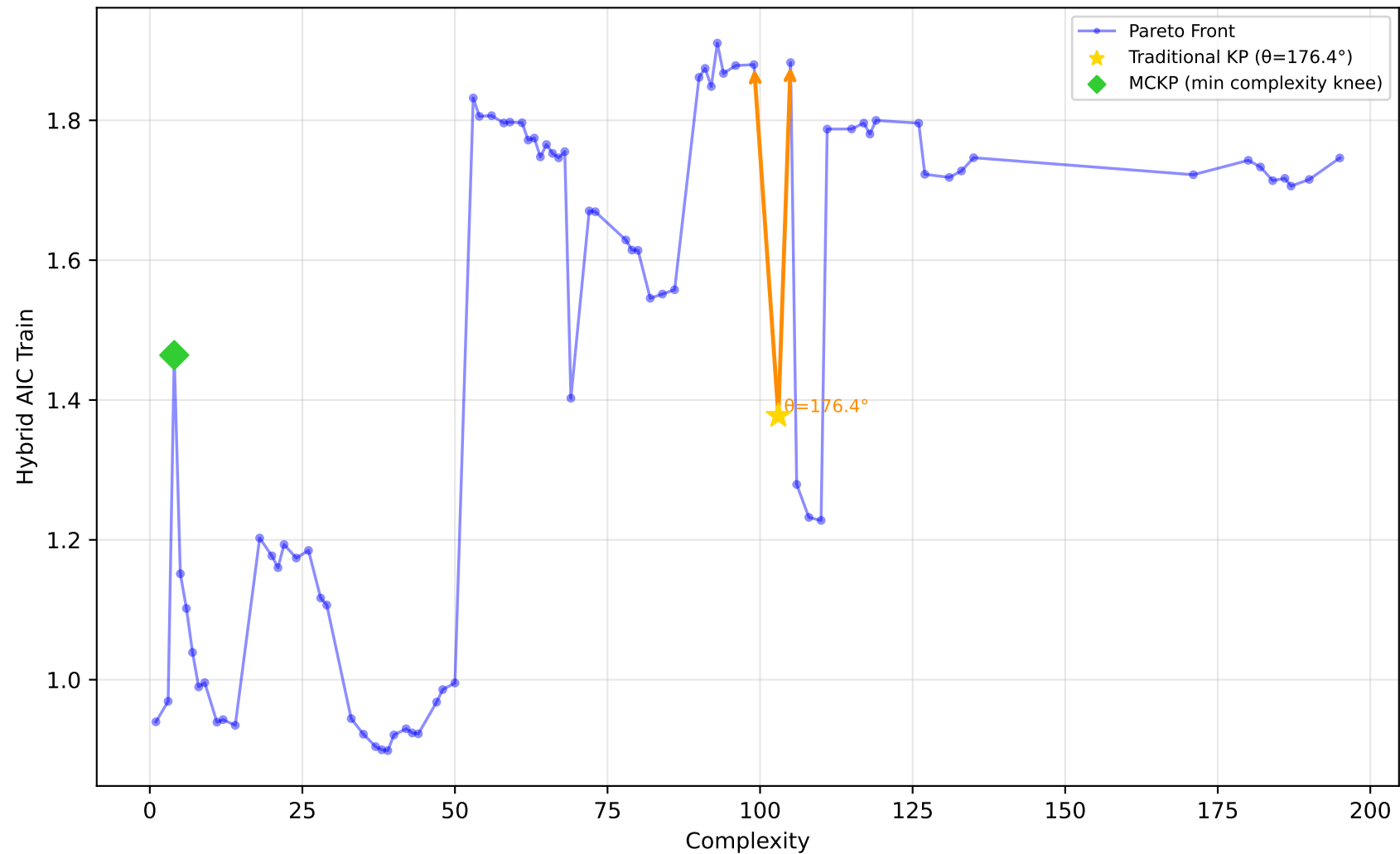
542_pollution - Run 14 - SVP - Hybrid AIC Train \lambda_1=0.70, \lambda_2=1.00, \lambda_3=0.10 | Difficulty: 1.00 | Method: hmr
