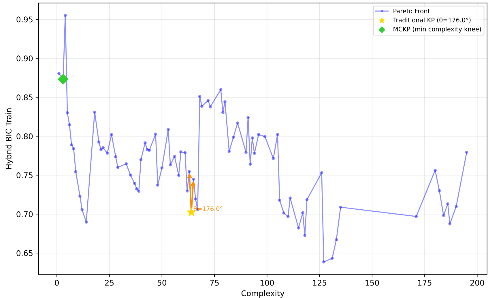
542_pollution - Run 14 - SVP - Hybrid BIC Train \lambda_1=0.00, \lambda_2=0.00, \lambda_3=0.20 | Difficulty: 1.00 | Method: hmr
