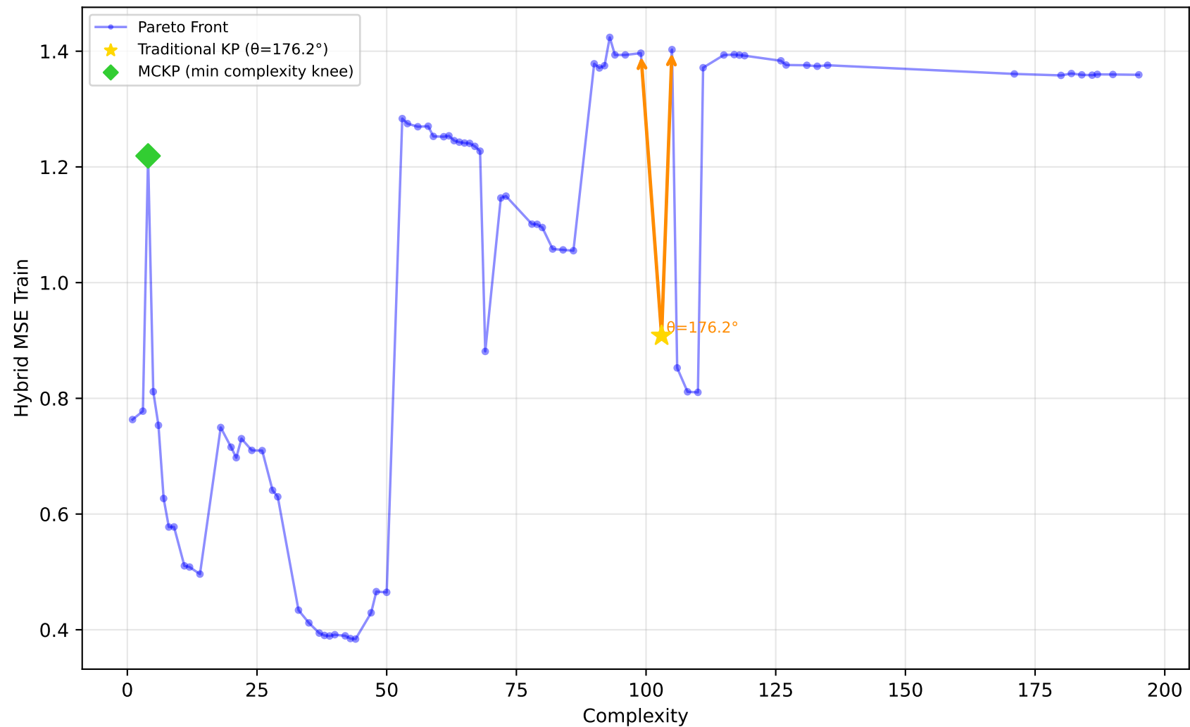
542_pollution - Run 14 - SVP - Hybrid MSE Train \lambda_1=0.70, \lambda_2=1.00, \lambda_3=0.10 | Difficulty: 1.00 | Method: hmr
