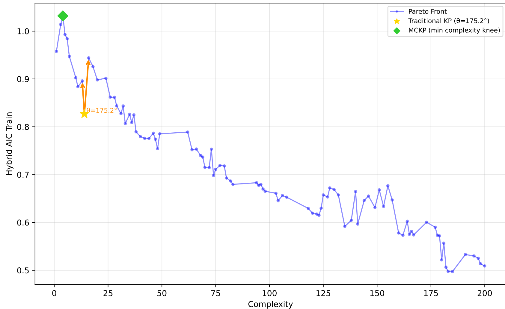
542_pollution - Run 15 - MVP - Hybrid AIC Train \lambda_1=1.00, \lambda_2=0.10, \lambda_3=0.00 | Difficulty: 0.42 | Method: mckp
