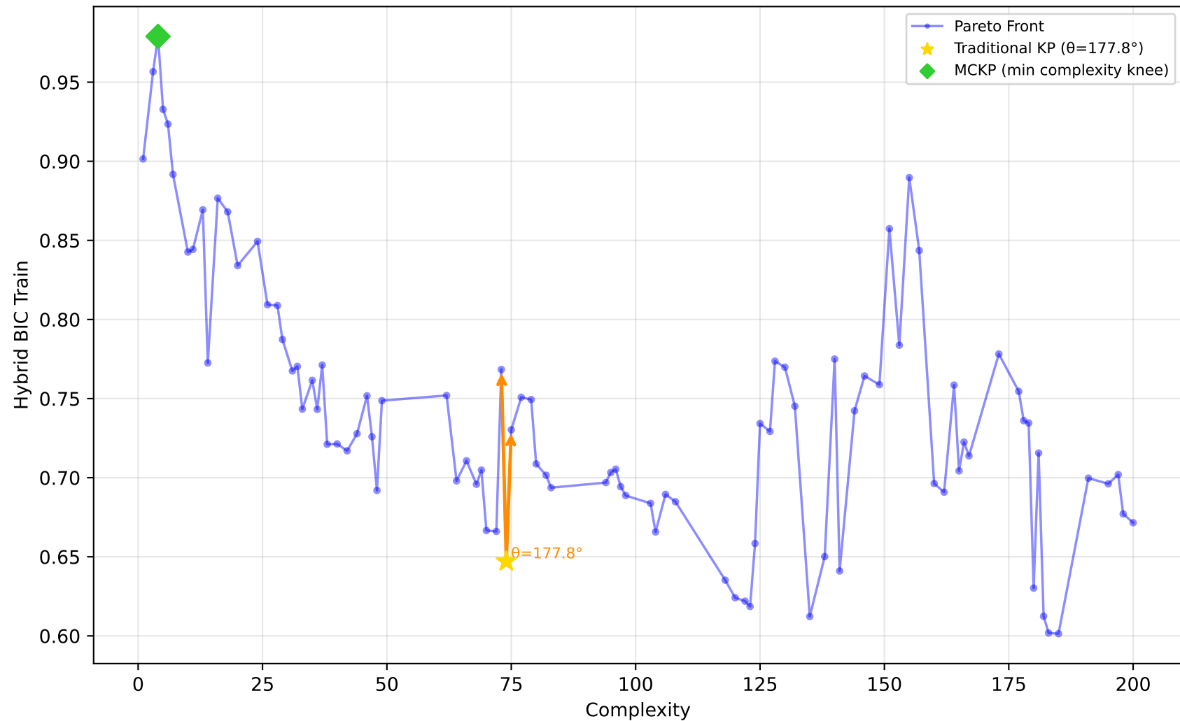
542_pollution - Run 15 - MVP - Hybrid BIC Train \lambda_1=1.00, \lambda_2=0.10, \lambda_3=0.00 | Difficulty: 0.42 | Method: mckp
