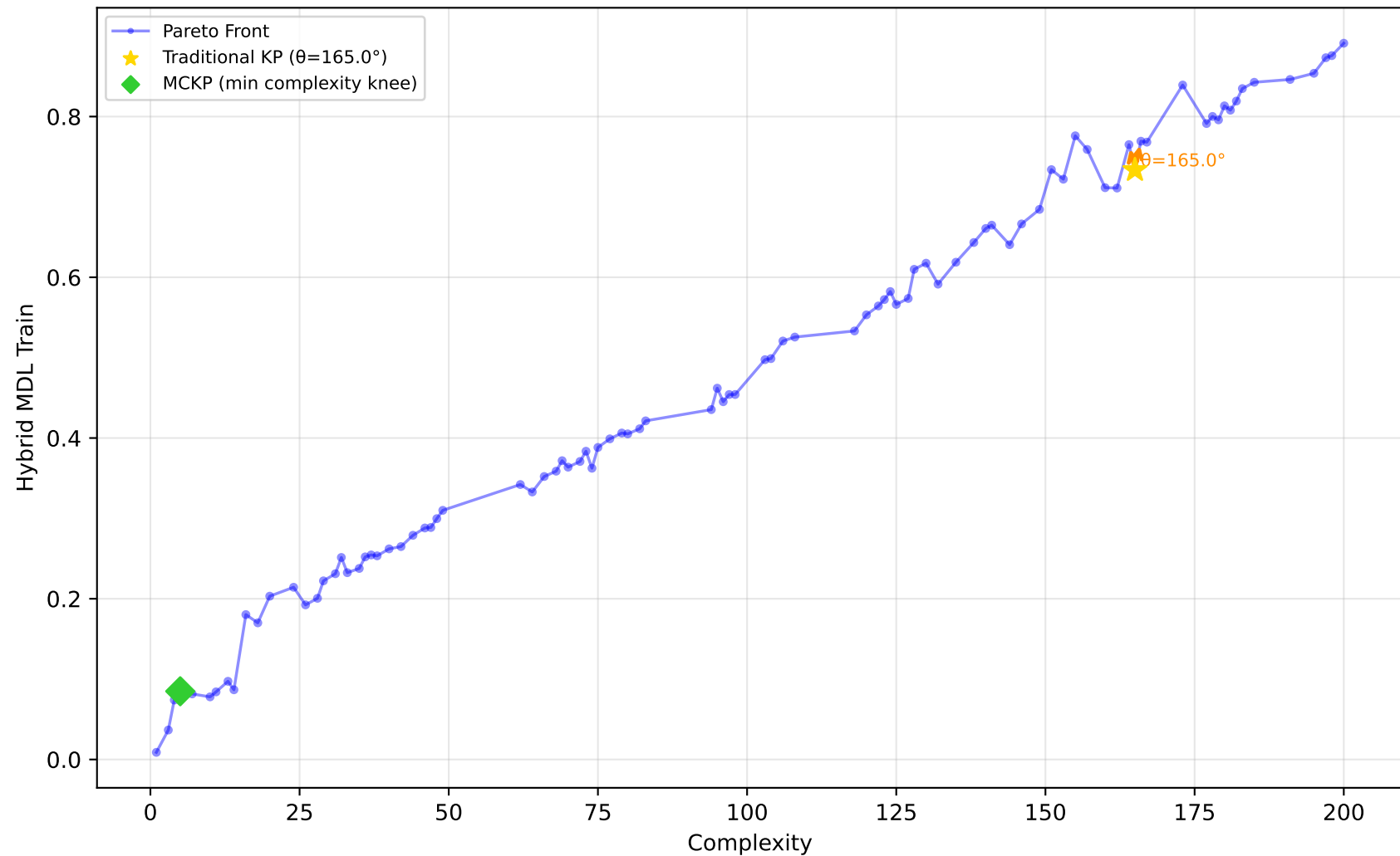
542_pollution - Run 15 - MVP - Hybrid MDL Train \lambda_1=0.40, \lambda_2=0.10, \lambda_3=0.00 | Difficulty: 0.42 | Method: mckp
