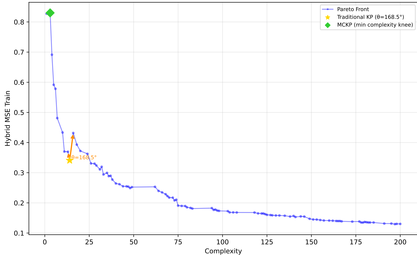
542_pollution - Run 15 - MVP - Hybrid MSE Train \lambda_1=0.40, \lambda_2=0.10, \lambda_3=0.00 | Difficulty: 0.42 | Method: mckp
